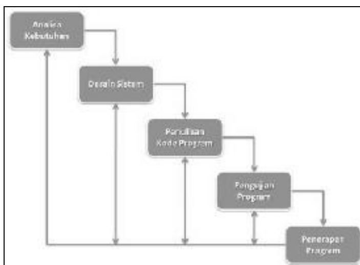
Gambar 1. Model Waterfall
